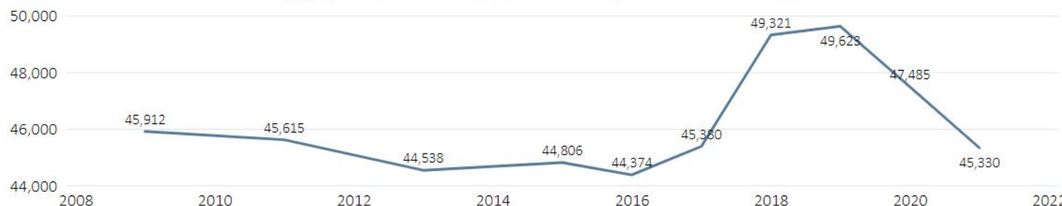
Utslipp (tonn CO 2 -ekvivalenter) 2009-2021 i Hitra
